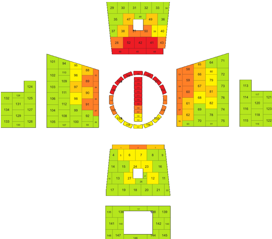
Wear Management, Liner Wear Map
